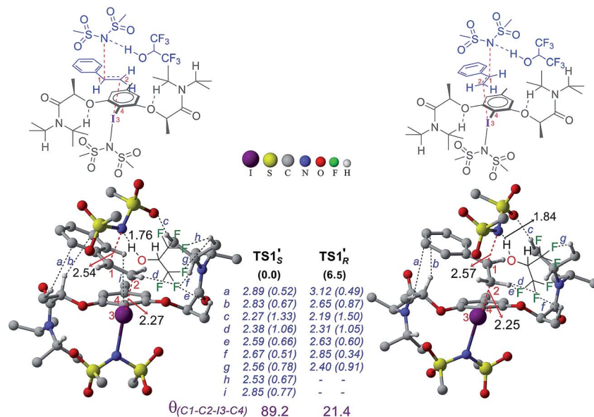
Fig. 6 Optimized geometries of the stereoselective transition states TS1 S and TS1 R . Relative Gibbs free energy is given in parentheses. Important noncovalent interactions (a–i) are shown in blue along with the corresponding electron densities ( \rho \times 10^{-2} au in parentheses) at the bond critical points along the bond paths. All distances are in Å.
