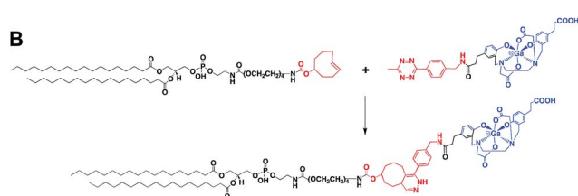
Fig. 4 (A) Radio-HPLC chromatograms of (top) ^{68}\text{Ga} -HBED-CC-tetrazine precursor and (bottom) reaction between 4 and 5 , after 15 min at 60 ^{\circ}\text{C} . (B) Scheme of the reaction between TCO-modified PE ( 4 ) and ^{68}\text{Ga} -HBED-CC-tetrazine ( 5 ).
