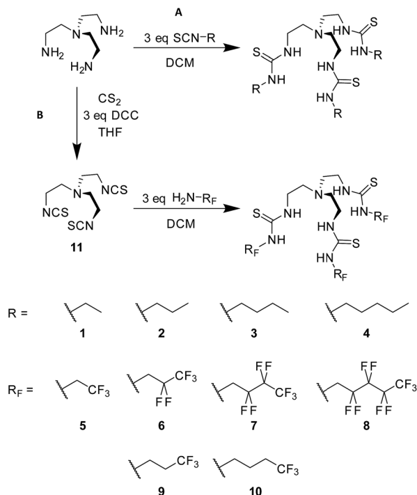
Fig. 1 Synthesis and general structure of the tris-thiourea series, (A) alkyl compounds 1–4, \text{SCN-R} = isothiocyanates; (B) compounds 5–10 with fluorinated alkyl ( \text{R}_\text{F} ) chains.
