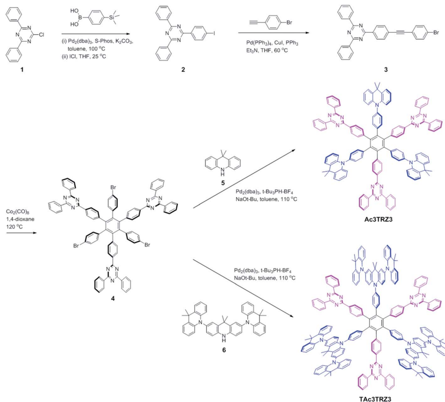
Scheme 1 Synthesis of the through-space charge transfer hexaarylbene Ac3TRZ3 and TAc3TRZ3.
