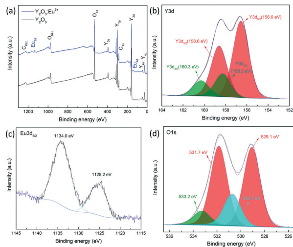
Fig. 5 (a) Full XPS spectrum of \text{Y}_2\text{O}_3:5\%\text{Eu}^{3+} nanoparticles annealed at 600 °C; (b) XPS spectrum of Y3d; (c) XPS spectrum of \text{Eu}^{3+}5/2 ; (d) XPS spectrum of O1s.
