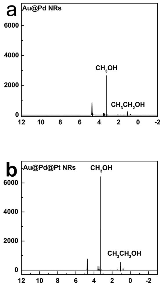
Fig. 6 Product analysis of \text{CO}_2\text{RR} on Au@2Pd (a) and Au@2Pd@0.5Pt (b) by NMR.
