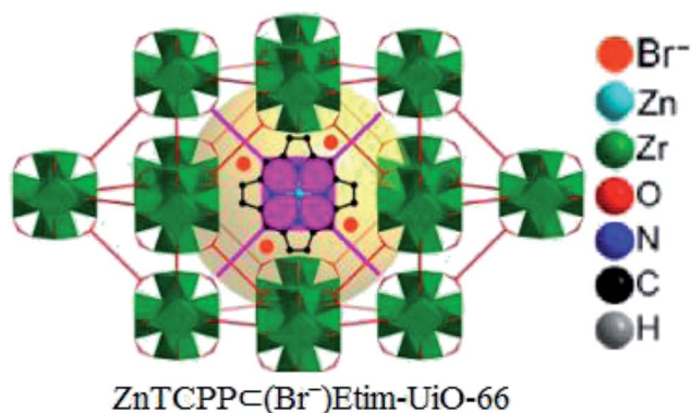
Fig. 8 Perspective view of structure of \text{ZnTCPP} \subset (\text{Br}^-)\text{Etim-UiO-66} .
