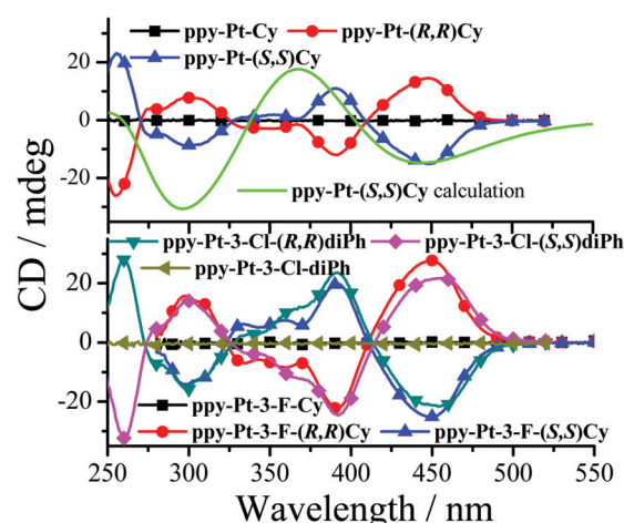
Fig. 10 Experimental CD spectra of ppy-Pt-(S,S)Cy , ppy-Pt-(R,R)Cy , racemic ppy-Pt-Cy , ppy-Pt-3-F-(S,S)Cy , ppy-Pt-3-F-(R,R)Cy , and racemic ppy-Pt-3-Cl-diPh ( 5.0 \times 10^{-5} mol dm -3 in MeCN). Computational CD spectra of ppy-Pt-(S,S)Cy (in THF).
