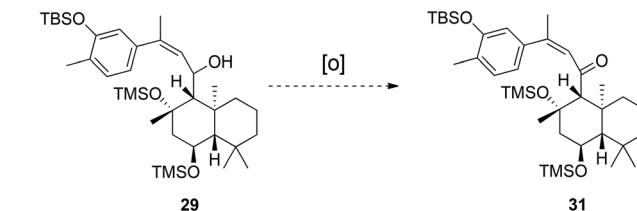
Scheme 6 Attempted oxidation of allylic alcohol 29.
