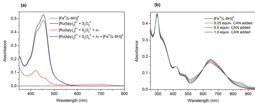
Fig. 2 (a) UV-vis spectra demonstrating the photochemical oxidation of [Ru(bpy) 3 ] 3+ (0.05 mM) to [Ru(bpy) 3 ] 3+ by persulfate (0.2 mM) with the following reduction by the catalyst [Fe V (L-6H)] - (0.5 μM). The spectrum of the catalyst (0.5 μM) is given for comparison in grey. (b) UV-vis spectra demonstrating titration of the catalyst [Fe IV (L-6H)] 2- (0.02 mM) by CAN.
