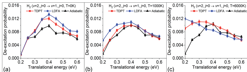
Fig. 7 Vibrational deexcitation probabilities from H 2 (v = 2, j = 0) to H 2 (v = 1, j = 0) simulated by MD, MDEF(LDFA), and MDEF(TDPT), with electronic temperatures of 0 K (a), 1000 K (b), and 6000 K (c).
