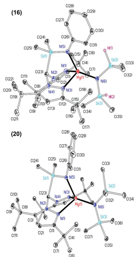
Fig. 2 Thermal displacement ellipsoid drawings (20% probability ellipsoids) of \text{Mg}(\text{HC}(\text{'Bu}_2\text{pz})_2\text{SiMe}_2\text{NPh})\{\text{N}(\text{SiHMe}_2)_2\} (16, top) and \text{Mg}(\text{HC}(\text{'Bu}_2\text{pz})_2\text{SiMe}_2\text{NPh})\{\text{N}(\text{SiMe}_3)_2\} (20, bottom). C-Bound hydrogen atoms have been omitted for clarity.
