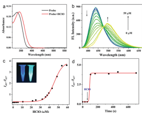
Fig. 1 (a) UV-vis absorption spectra of the probe TPA-CIO with and without excessive HClO. (b) Fluorescence spectra of 10 \mu\text{M} TPA-CIO in the presence of HClO (0–59 \mu\text{M} ). (c) Plot of the fluorescence emission ratio ( I_{497}/I_{437} ) of TPA-CIO versus [HClO] (0–59 \mu\text{M} ). Inset: Photograph of TPA-CIO before and after reacting with HClO under 365 nm excitation. (d) Time dependence of the fluorescence emission ratio ( I_{497}/I_{437} ) for 10 \mu\text{M} TPA-CIO in the presence of excessive HClO (60 \mu\text{M} ). The measurements were carried out in PBS/DMF (v : v = 1 : 1, pH 7.4, 10 mM) solution. Reaction time: 60 s.
