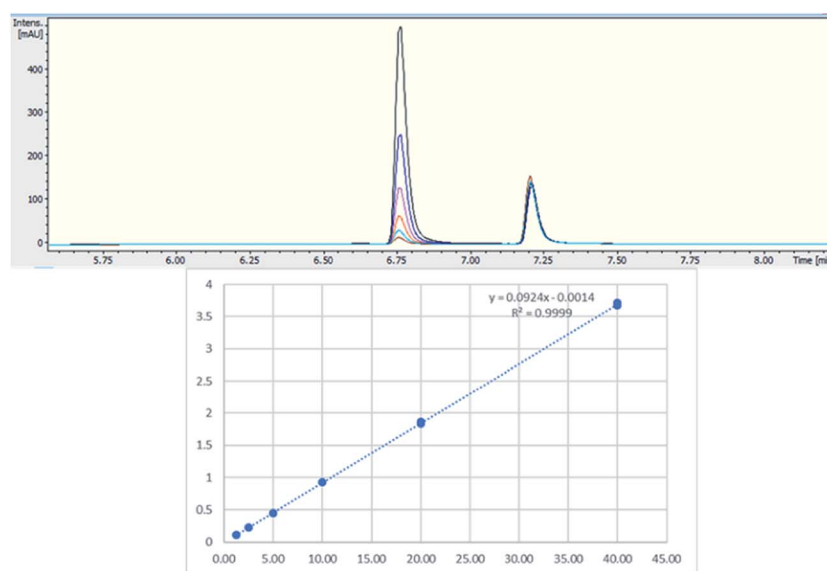
Fig. 4 (Upper) stacked UHPLC chromatogram concentrations from 1.25 to 40.0\text{ }\mu\text{g mL}^{-1} ( \lambda = 298\text{ nm} ) of 5F-ADB ( \text{RT} = 6.8\text{ min} ) and 5F-AKB48 IS ( \text{RT} = 7.2\text{ min} ); (lower) calibration curve of 5F-ADB against 5F-AKB48 (IS), R^2 = 0.9999 .
