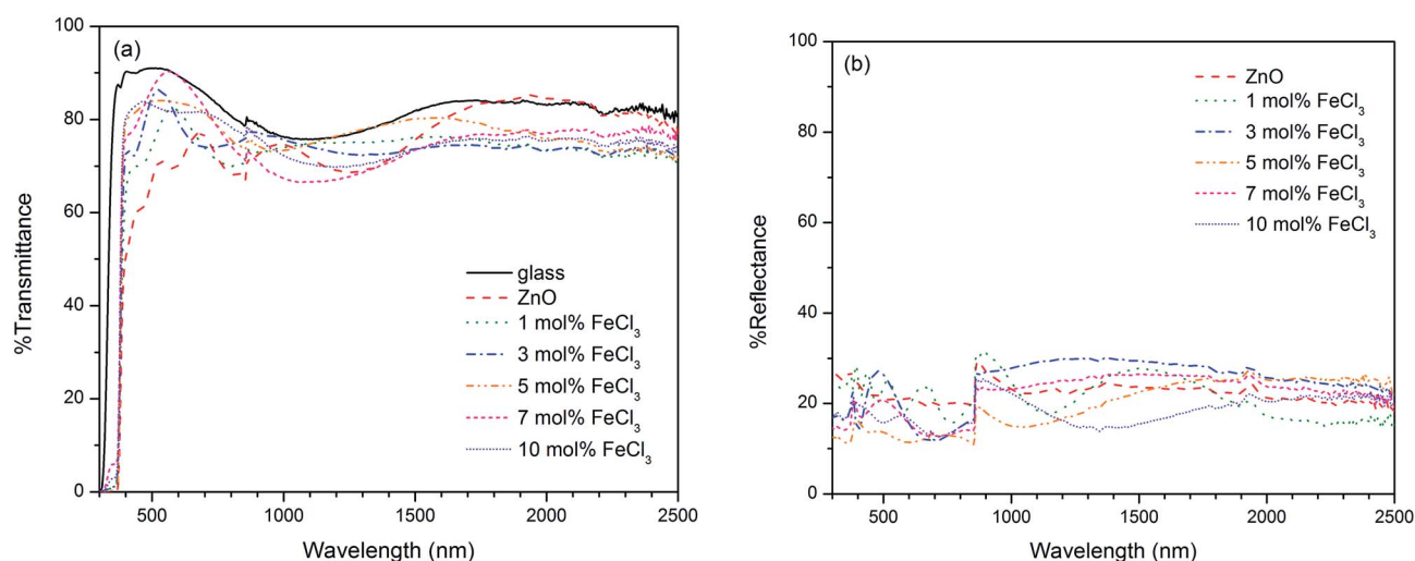
Fig. 9 (a) Transmittance and (b) reflectance spectra of all films and the spectrum of bare glass was collected as reference. ZnO:Cl films improve % T from carbon-contaminated undoped ZnO film. The films with 7 mol% FeCl 3 exhibits the highest % T of 85.
