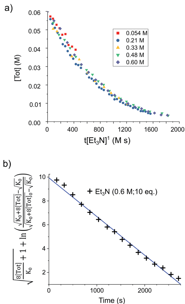
Fig. 3 (a) Solutions of 1 (0.03 mmol) in d_8 -toluene (0.5 mL) under \text{H}_2 (4 bar) containing various base concentrations were prepared. When the stannylene concentration, [\text{Tot}] , is plotted against the normalised timescale t \cdot [\text{Et}_3\text{N}]^1 , all traces overlap, confirming the order in base to be one. (b) Linearised rate data for a similar solution of 1 (0.03 mmol) in d_8 -toluene (0.5 mL) under \text{H}_2 (4 bar) containing \text{Et}_3\text{N} (0.6 M; 10 eq.).
