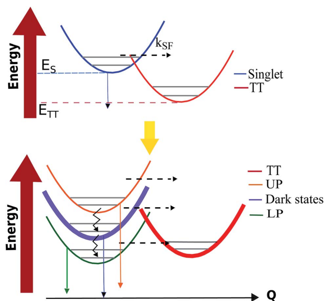
Fig. 7 Scheme of the transfer processes relevant to SF under normal (top) and strong coupling (bottom) conditions. Solid (jagged) arrows indicate radiative (nonradiative) decay processes. Dashed arrows account for transitions between states with different electronic character. Thicker lines indicate larger DOS.
