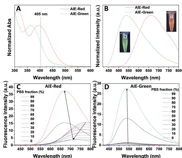
Fig. 1 The normalized absorption (A) and fluorescence (B) spectra of AIE-Red (10 μM) and AIE-Green (10 μM) in PBS buffer (pH = 7.4, containing 0.5% DMSO). The insets show the optical photographs of these solutions obtained under 365 nm light irradiation. (C and D) Fluorescence spectra of AIE-Red (10 μM, (C)) and AIE-Green (10 μM, (D)) in DMSO/PBS mixtures with different volume fractions of PBS from 0 to 99%. The excitation wavelength was 405 nm for all the fluorescence spectra.
