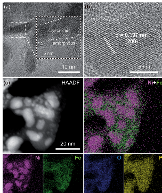
Fig. 2 (a) TEM image, (b) HRTEM image, (c) HAADF-STEM image and EDS elemental mapping images for the \text{Ni}_2\text{P}@ \text{FePO}_x sample.
