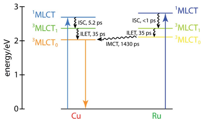
Fig. 8 Jablonski diagram for CuMe 2 -RuH 2 with the copper- and ruthenium-centered states shown on the left and right sides, respectively. The energies of both 1 MLCT states and the copper-centered 3 MLCT 0 state are estimated from steady-state absorption and emission measurements, and all other energies are qualitative estimates.
