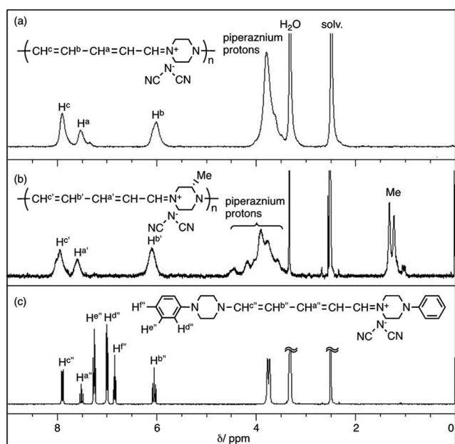
Fig. 1 1 H NMR spectra of polymer(H;(CN) 2 N - ) , polymer(S-Me;(CN) 2 N - ) and model(H;(CN) 2 N - ) in DMSO- d 6 .
