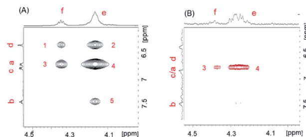
Fig. 4 NOESY spectra of 2 wt% 5'DSCG with (A) and without (B) LB components in \text{D}_2\text{O} . With LB, cross peaks 1, 2, and 5 are intermolecular NOEs, and 3 and 4 are a mixture of inter- and intramolecular NOEs. Without LB, cross peaks 3 and 4 are intramolecular NOEs.
