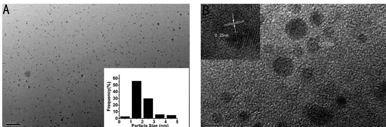
Fig. 3 (A) TEM image of as-prepared p53 probe 1/p53-Ag NCs with an average diameter of 2\text{ nm} (inset: the size distribution histograms of the DNA-Ag NCs); (B) high-resolution TEM image of p53 probe 1/p53-Ag NCs (inset: the amplified image).
