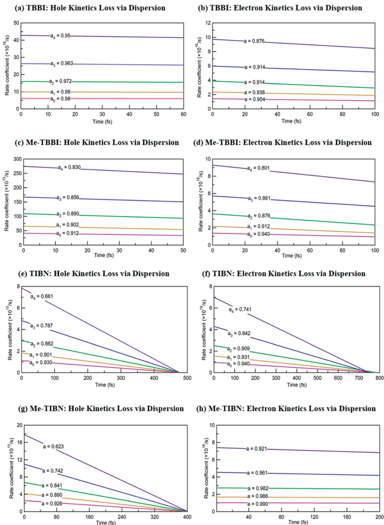
Fig. 6 The dispersive parameters ( a_0, a_1, a_2, a_3 and a_4 ) at different applied fields of 0, 7.144 \times 10^3, 1.428 \times 10^4, 2.143 \times 10^4 and 2.857 \times 10^4 V cm ^{-1} for hole and electron transport in TBBI, Me-TBBI, TIBN and Me-TIBN molecules.
