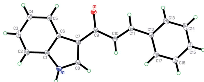
ORTEP of the synthesized compound 1a
