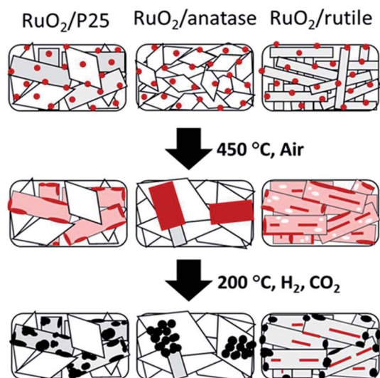
Fig. 5 Schematic illustration of the shape evolution of \text{RuO}_2/\text{TiO}_2 catalysts: after \text{RuO}_2 nanoparticle deposition, after thermal annealing at 450 °C, and after reduction and methanation. Red indicates \text{RuO}_2 , pink indicates thin \text{RuO}_2 layer, white indicates Ru depleted area, and black indicates metallic Ru. Reprinted with permission from ref. 67. Copyright 2013 RSC.
