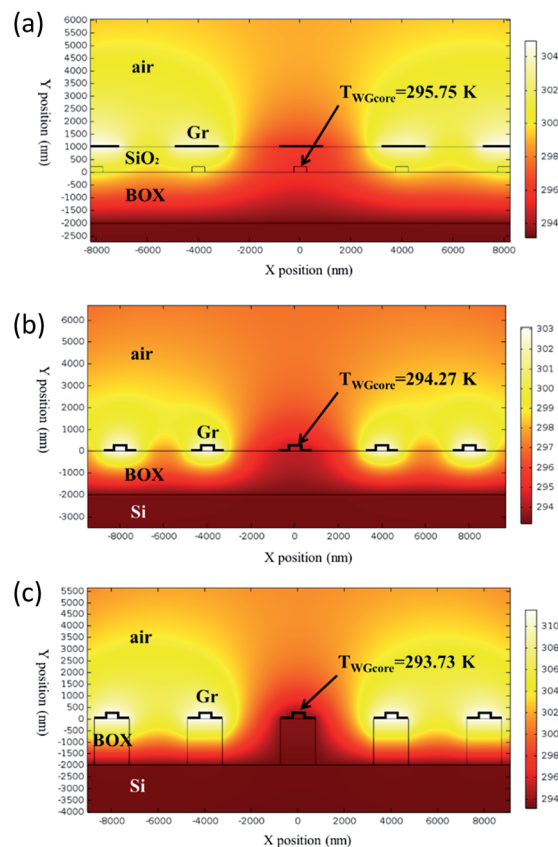
Fig. 11 Thermal field distributions of conventional structure with 1 \mu\text{m} -thick \text{SiO}_2 top cladding (a), graphene contact-heating structure without air trench (b) and with air trench (c).
