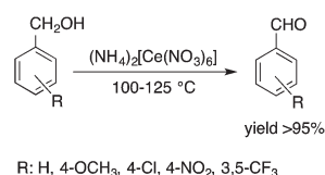
Scheme 13 Oxidation of benzyl alcohol and its derivatives.
