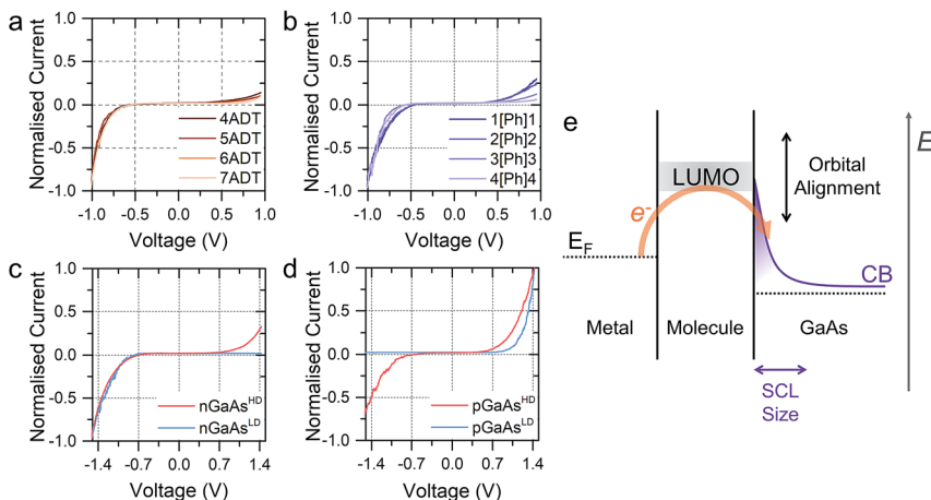
Fig. 2 (a) I – V characteristics of \alpha,\omega -alkanedithiols of increasing length on n\text{GaAs}^{\text{HD}} . (b) I – V characteristics of the \text{X}[\text{Ph}]\text{X} series on n\text{GaAs}^{\text{HD}} . (c) I – V characteristics of 5ADT on n\text{GaAs} of different doping concentration. (d) I – V characteristics of 5ADT on p\text{GaAs} of different doping concentration. (e) Band diagram for the reverse biased junction with n\text{GaAs} , where E is the electron energy. All data shown in this Figure is obtained in the dark. Note that the sense corresponding to forward bias is opposite between panel c and d. Junctions made at n -type \text{GaAs} have forward bias at negative potential, and junctions made at p -type \text{GaAs} have forward bias at positive potential.
