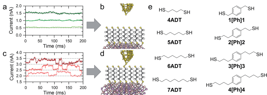
Fig. 1 (a) Tunneling readout at low setpoint bias, where the tip is not in contact with the monolayer, as depicted in (b). (c) Tunneling readout at higher setpoint bias, where the sudden jumps are related to the formation of Au-S bonds between the tip and the monolayer thiolated termini (d). (e) Structure of molecular wires employed in this study.
