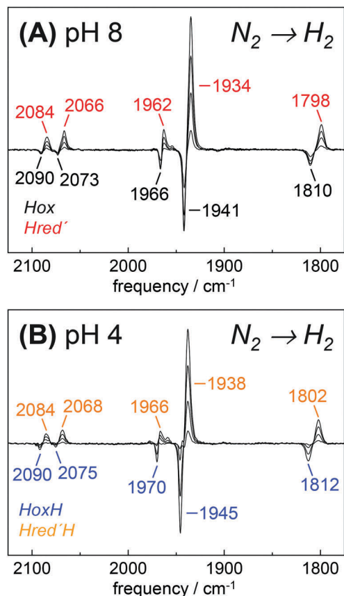
Fig. 7 Reduction of \text{HYDA1}^{\text{Pdt}} in the presence of \text{H}_2 . IR difference spectra collected during a change in the aerosol from \text{N}_2 to \text{H}_2 . (A) At pH 8 and 2 mM DT, Hox (black) was found to be de-populated in favor of Hred' (red). (B) At pH 4 and 2 mM DT, HoxH (blue) converted into Hred'H (orange).
