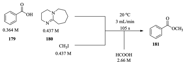
Scheme 35 Scaled up alkylation of benzoic acid by Mel in the presence of 1,8-diazabicyclo[5.4.0]-undec-7-ene (DBU) in a Corning low flow reactor.
