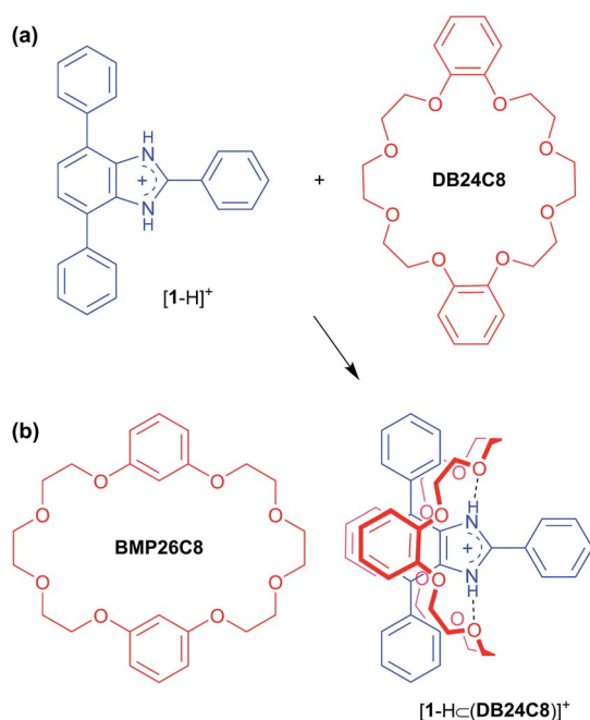
Scheme 1 (a) The [2]pseudorotaxane, [1-H \subset \text{DB24C8}]^+ can be formed via supramolecular interactions (ion-dipole, hydrogen-bonding and \pi -stacking) between the T-shaped benzimidazolium cation, [1-H]^+ and the 24-membered crown ether DB24C8 . 17,18a (b) Of relevance to this work, the crown ether BMP26C8 can also form a similar [2]pseudorotaxane, [1-H \subset \text{BMP26C8}]^+ with [1-H]^+ . 18b
