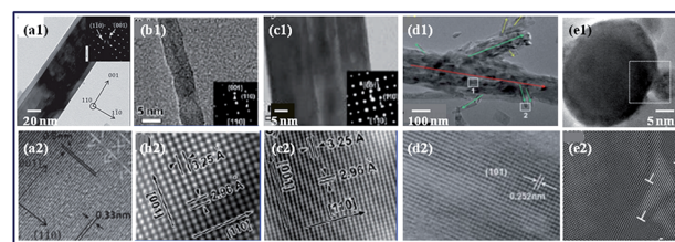
Fig. 17 TEM/HR-TEM micrographs of rutile-TiO 2 nanostructures: (a 1 and a 2 ) TEM image and corresponding HR-TEM image of a nanobelt, 290 (b 1 and c 1 ) TEM images of one individual nanowire and nanorod, 271 (b 2 and c 2 ) corresponding HR-TEM images of the nanowire and nanorod, 271 (d 1 and d 2 ) low magnification TEM and HR-TEM images of multilevel branched architectures, 286 (e 1 ) the lattice image and (e 2 ) reconstructed image from the square region in (e 1 ). 294 Insets (in a 1 , b 1 and c 1 ) illustrate the corresponding SAED patterns. (a 1 and a 2 ) are reprinted with permission from ref. 290. Copyright 2015. John Wiley and Sons. (b 1 , b 2 , c 1 and c 2 ) are reprinted with permission from ref. 271. Copyright 2011. American Chemical Society. (d 1 and d 2 ) are reprinted with permission from ref. 286. Copyright 2012. The Royal Society of Chemistry. (e 1 and e 2 ) are reprinted with permission from ref. 294. Copyright 2004. Nature Publishing Group.
