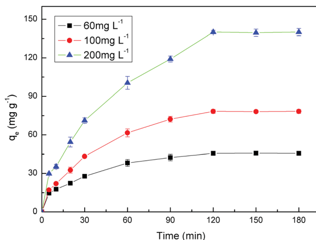
Fig. 7 Effect of contact time on U(vi) adsorption. (Volume, 30 mL; absorbent dose, 0.03 g; initial concentration, 60, 100 and 200 mg L -1 ; pH value, 4.0; contact time, 0, 5, 10, 20, 30, 60, 90, 120, 150, 180 min; temperature, 25 °C; rotating speed, 150 rpm.)
