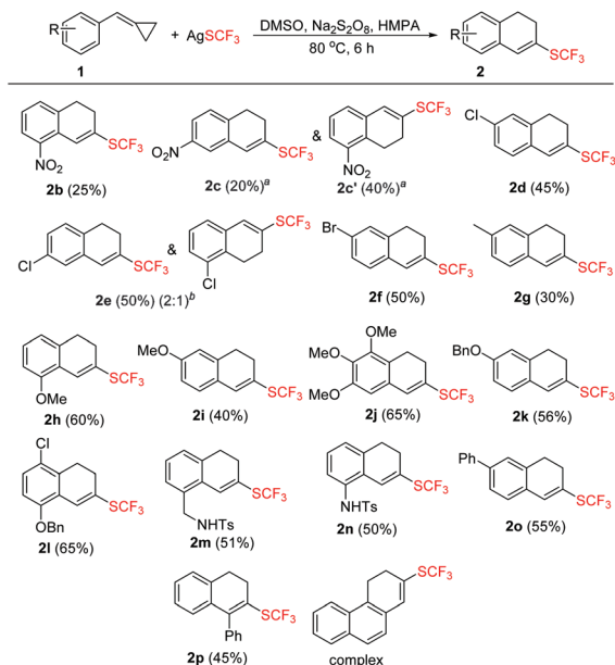
Scheme 2 Substrate scope of 1 . The reaction conditions: 1 (0.6 mmol), \text{AgSCF}_3 (0.2 mmol), \text{Na}_2\text{S}_2\text{O}_8 (0.6 mmol), and \text{HMPA} (0.1 mmol) were dissolved in 3 mL \text{DMSO} and the reaction mixture was stirred at 80^\circ\text{C} for 6 h. All the yields are isolated yields and \text{AgSCF}_3 was taken as a standard for yield evaluation. a The two isomers can be separated. b The two isomers cannot be isolated.
