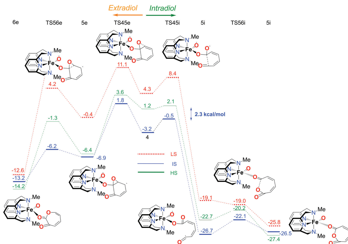
Fig. 7 Calculated reaction profile for the second part of the catalytic mechanism with the LN 4 Me 2 ligand, branching to the extradiol (left) and intradiol (right) pathways. Electronic energies (kcal mol -1 ), obtained using the S12g/TZ2P level of theory, are given relative to reactants.
