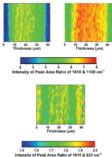
Fig. 4 The Raman cross-sectional microscopic maps of the desiccator-dried RG-AEM( \text{Cl}^- )s: top-left map = LDPE-AEM (50 kGy), top-right map = LDPE-AEM (100 kGy), and bottom map = ETFE-AEM (30 kGy). The through-plane (AEM thickness) direction is on the x-axes. The 1610 \text{ cm}^{-1} Raman peak is from the benzene rings on the functional graft chains, the 1130 \text{ cm}^{-1} Raman peak relates to the LDPE precursor material, and the 833 \text{ cm}^{-1} peak relates to the ETFE precursor material. A laser of 532 \text{ nm} wavelength ( 8 \text{ mW} power) and a 50\times objective was used giving a spatial resolution of \text{ca. } 1 \mu\text{m} diameter.
