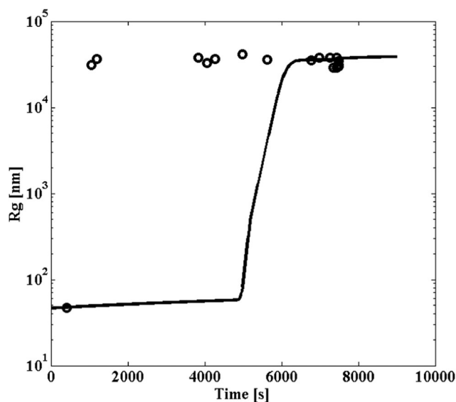
Fig. 6 Radius of gyration evolution as a function of time, for particle volume fraction equal to 21% and shear rate of 1700 \text{ s}^{-1} . The points are experimental data, while the line is the corresponding model predictions, in the case where the aggregation is modeled by kernel (2). The calculations have been carried out with the stability ratio value W = 10^8 .
