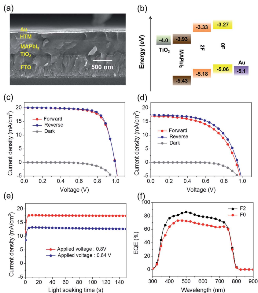
Fig. 7 (a) The SEM cross-sectional image and (b) energy diagram of the perovskite solar cell device. The current density–voltage ( J – V ) characteristics based on the solar cells with (c) 2F and (d) 0F . (e) current density ( J ) variation of the 0F and 2F based PSCs with a light soaking (1 Sun) time under the applied bias voltage ( V_{opt} ) at maximum power point ( P_{max} ) and (f) EQE spectra of the 0F and 2F based PSCs.
