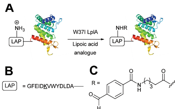
Scheme 6 (A) Outline of using Lipolic acid ligase (LplA) mutants for installing aldehydes into LplA acceptor peptide (LAP) bearing proteins. (B) Amino acid sequence of the LAP. (C) Structure of the incorporated aldehyde.
