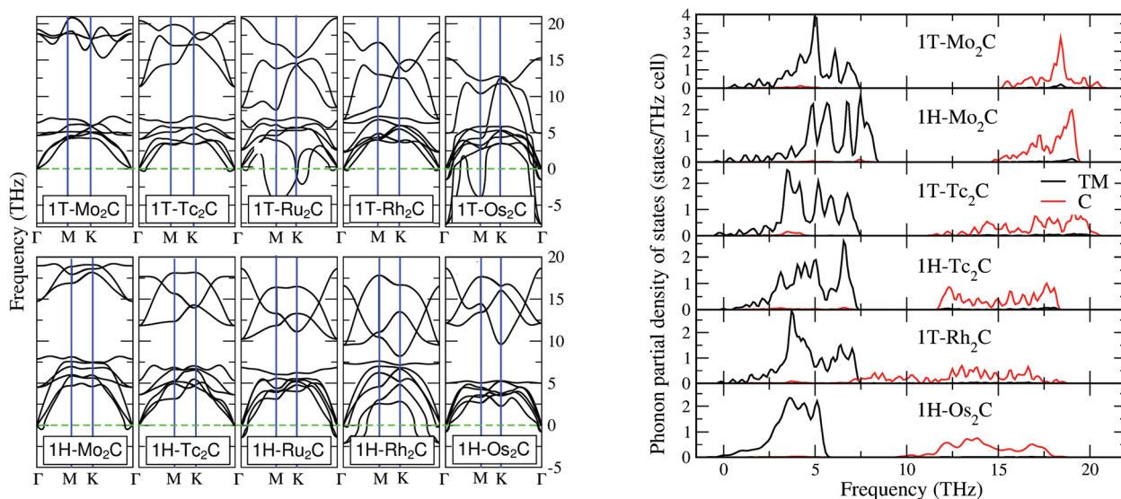
Fig. 2 Left panel: The phonon dispersion curves for the single layer of \text{M}_2\text{C} \text{M} = \text{Mo, Tc, Ru, Rh, Os} with both 1T and 1H symmetries. Right panel: The phonon site-projected density of states (PSPDOS) of 1T-Mo 2 C, 1H-Mo 2 C, 1T-Tc 2 C, 1H-Tc 2 C, and 1T-Rh 2 C and 1H-Os 2 C (from top to bottom).
