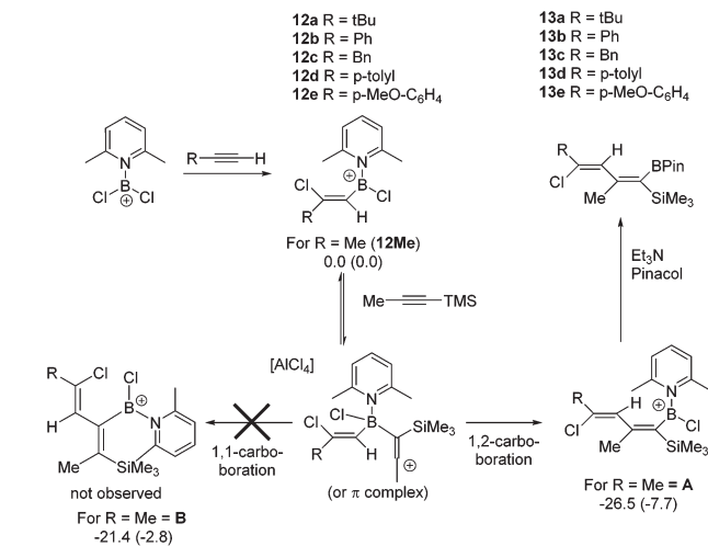
Scheme 4 1-Boradiene formation by haloboration and 1,2-carboboration. Electronic energies (Gibbs free energies at 293 K) shown in kcal mol -1 for the model system where R = Me (all energies relative to 12Me and 1-TMS-1-propyne at infinite distance).
