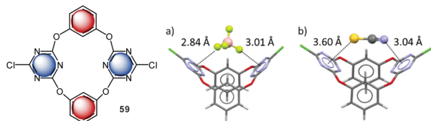
Fig. 33 Molecular structure of the anion receptor as investigated by Wang's group. The solid state structures of the co-crystals with corresponding tetraalkylammonium salts demonstrate anion-π interactions between the anions and the electron deficient triazine moiety.
