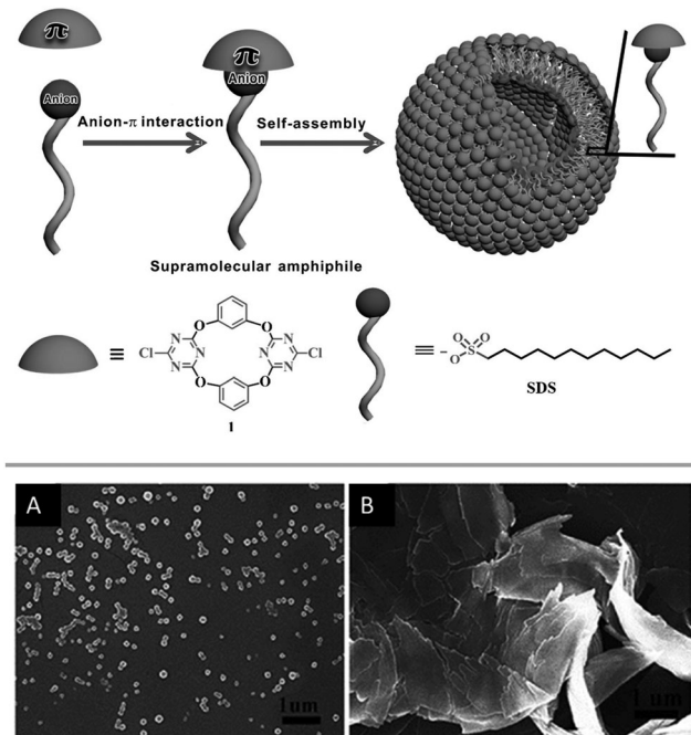
Fig. 34 Schematic representation of the anion-π induced self-assembly forming the vesicle as well as SEM images before (A) and after addition of 3 eq. of NaNO 3 (B). Reproduced with permission from John Wiley and Sons. 66
