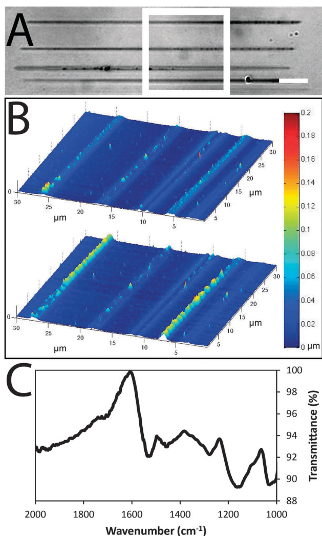
Fig. 2 (A) Optical microscope image of black polypyrrole wires. The dotted white outline represents the scan area for AFM images, and the white scale bar represents 10 \mu m. (B) AFM image of wires in dry (top) and hydrated (bottom) states. (C) FTIR spectrum of CSA-doped polypyrrole.
