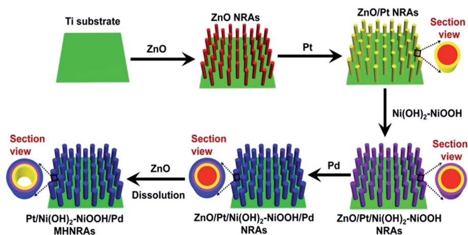
Scheme 1 Fabrication of the \text{Pt}/\text{Ni}(\text{OH})_2\text{-NiOOH}/\text{Pd} MHNRA.
