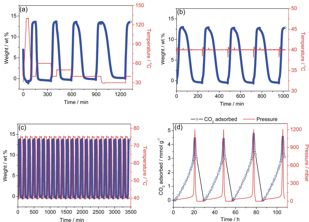
Fig. 3 (a) Adsorption-desorption cycling of CO 2 for 1-dmen, showing reversible uptake from simulated flue gas (0.15 bar CO 2 balanced with N 2 ). Adsorption temperature was 40 °C and desorption temperatures were 130 °C, 60 °C, 50 °C, 40 °C, and 30 °C under Ar. (b) Adsorption-desorption cycling of CO 2 at 40 °C by switching atmospheres between simulated flue gas and Ar. (c) Adsorption-desorption cycling of CO 2 at adsorption (40 °C) and desorption (75 °C) under Ar. (d) Vacuum-swing adsorption at 25 °C using a Micromeritics ASAP2020 instrument.
