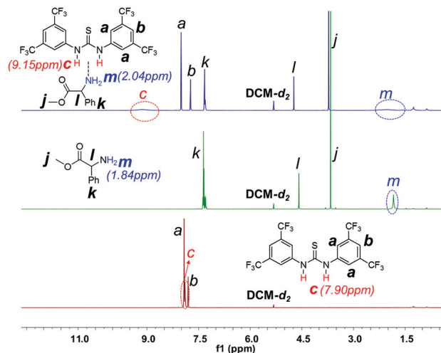
Fig. 7 ^1\text{H} NMR spectra of TU-S, methyl 2-amino-2-phenylacetate (MAP) and TU-S/MAP mixture (500 M, 25^\circ\text{C} , \text{CD}_2\text{Cl}_2 , for full spectrum of the mixture see Fig. S13 \dagger ).
