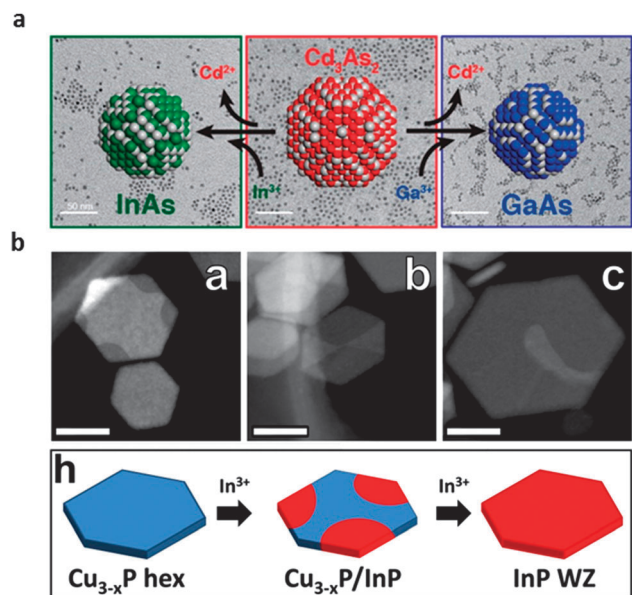
Fig. 2 (a) Illustration of the cation exchange reaction used to produce monodisperse III–V NCs (including GaAs, InAs, GaP, and InP) by substitution of group 13 ions in cadmium chalcide NCs. Reproduced with permission from ref. 21. (b) Preparation of hexagonal WZ InP NPLs via a cation exchange of \text{Cu}_{3-x}\text{P} with \text{In}^{3+} . Adapted with permission from ref. 22.
