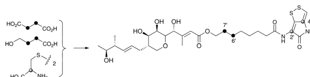
Scheme 2 Incorporation of [ ^{13}\text{C} ]-labelled succinate, 4-hydroxybutyrate and cystine into thiomarinol A.
