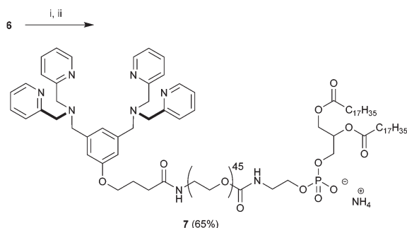
Scheme 2 Preparation of BDPA-PEG 2000 -DSPE ( 7 ). Conditions: (i) PfpOH, EDC, DMAP, \text{CHCl}_3 , 0^\circ\text{C} to rt, 16 h followed by (ii) \text{H}_2\text{N} -PEG 2000 -DSPE, DIPEA, \text{CHCl}_3 , rt, 24 h.
